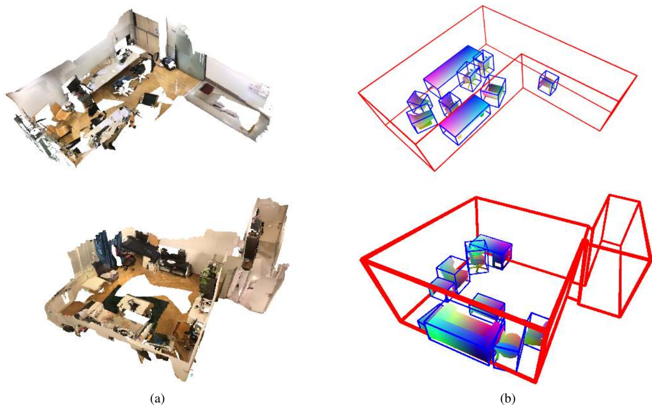
Figure 10: RGB-D scans of the authors' office and apartment (a) and the automatically retrieved object models from the full ShapeNet dataset and layout (b). Our method generalizes well to RGB-D scans outside the ScanNet dataset. Note the large areas with missing data, in particular for the layout.
