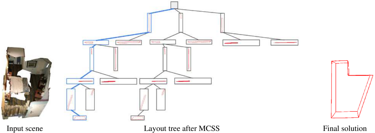
Figure 2: The layout proposals are organized into a tree structure such that proposals at the same level of the tree are incompatible to each other but compatible with proposals of their ancestor nodes. Our MCSS approach builds the search tree online and efficiently finds the optimal path, outlined blue, without exploring all candidate solutions.
