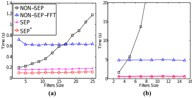
Fig. 5: Time needed to compute convolutions using a multi-thread MATLAB implementation, as a function of the filters size. (a) An image of 488 \times 488 pixels is convolved with a filter bank of J = 121 non-separable filters and K = 25 separable ones. (b) A volume of 114 \times 114 \times 50 voxels is convolved with a filter bank of J = 121 non-separable filters and K = 25 separable ones. Using parallel computation the time needed to compute the convolution is further reduced and our methods are still the most efficient ones. The times are averaged over 5 repetitions.
