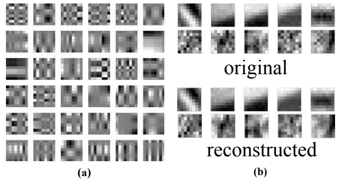
Fig. 7: Approximating an existing filter bank. (a) The 36 separable filters learned by SEP-COMB to approximate a bank of 256 filters learned with the K-SVD algorithm of [13]. (b) Comparison between some of the original filters learned by K-SVD (top row) and their approximations reconstructed by our algorithm (bottom row). While filters with a regular structure are very well approximated, noisy filters are slightly smoothed by the approximation. Their role in the denoising process is, however, marginal, and therefore this engenders no performance penalty.
